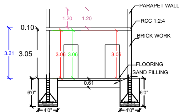
SECTION AB
