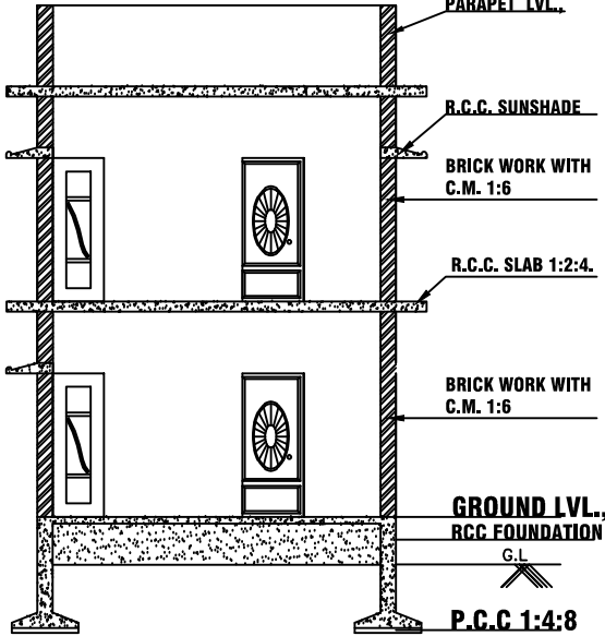
SECTION ON A-A & A'-A'
