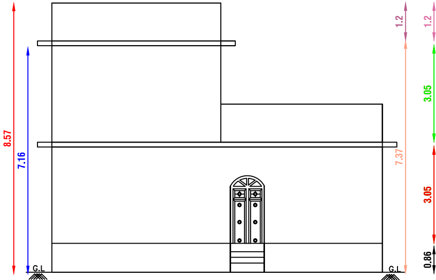
FRONT ELEVATION
