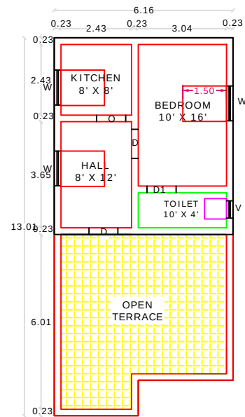
PROPOSED FIRST FLOOR RESIDENTIAL PLAN
