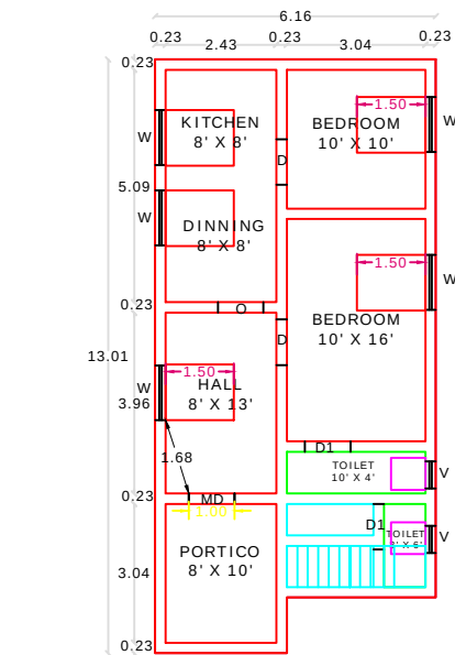
EXITING GROUND FLOOR RESIDENTIAL PLAN
