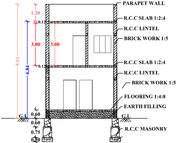
"SECTION 'AB'"
