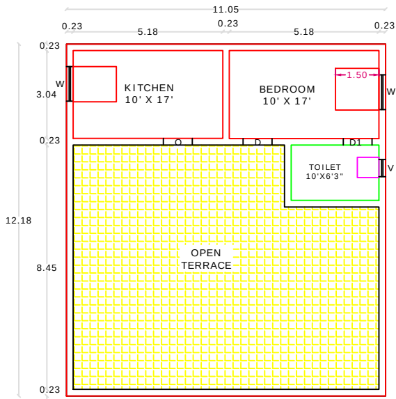
FIRST FLOOR RESIDENTIAL PLAN
