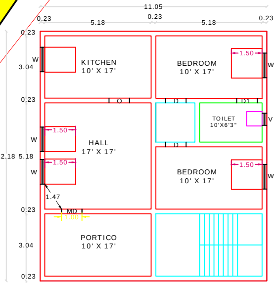
GROUND FLOOR RESIDENTIAL PLAN
