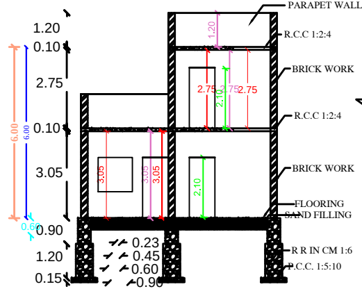
SECTION AB
