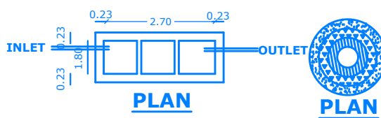
SEPTICTANK DETAILS
