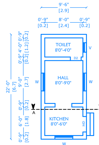
PROPOSED PLAN
