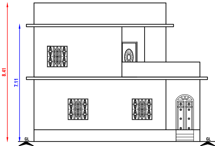
FRONT ELEVATION
