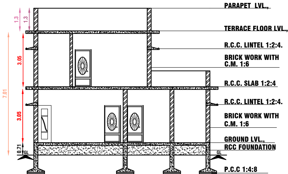
SECTION ON A-A & A'-A'
