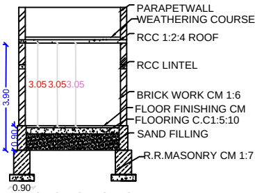
SECTION ON SV
