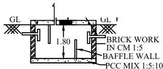
SECTION ON SEPTICTANK
