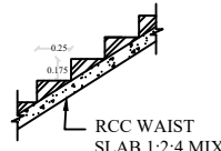
STAIR CASE DETAILS
