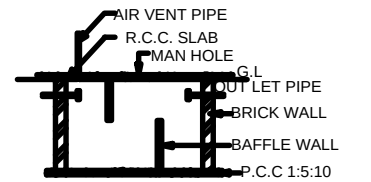
SECTION ON SEP.TANK
