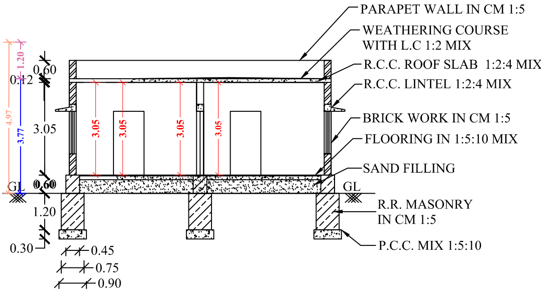
SECTION OF "BS"
