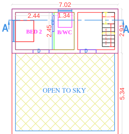
PLAN - FIRST FLOOR ( PROPOSED )
