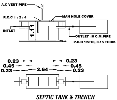
SEPTIC TANK & TRENCH
