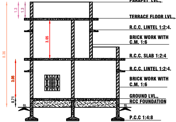
SECTION ON A-A & A'-A'
