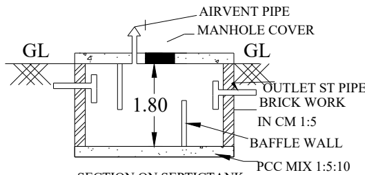
SECTION ON SEPTICTANK
