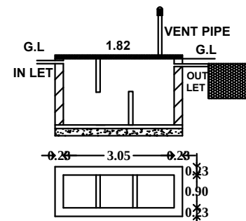
SEPTICTANK DETAILS
