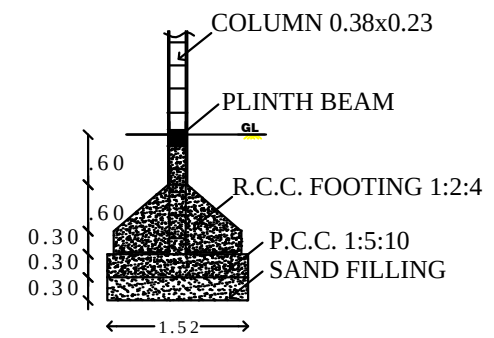
COLUMN DETAILS
