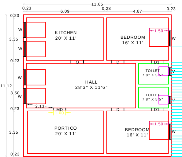
GROUND FLOOR IDENTIAL PLAN
