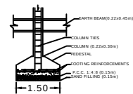
FOUNDATION DETAILS
