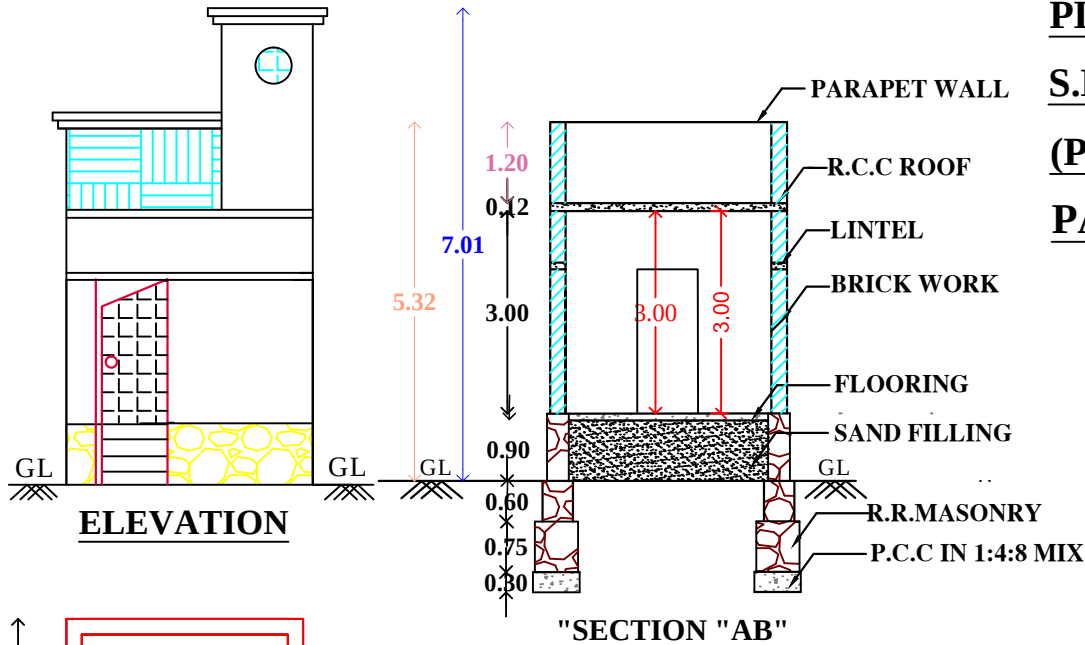
"SECTION "AB"
