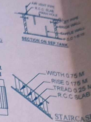
STAIRCASE
