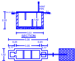
PLAN OF SEPTIC TANK AND TRENCH DETAILS
