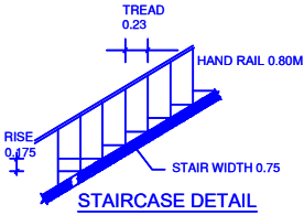
STAIRCASE DETAIL
