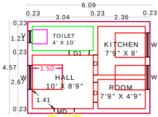
GROUND FLOOR RESIDENTIAL PLAN
