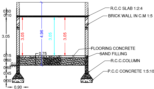
SECTION AB
