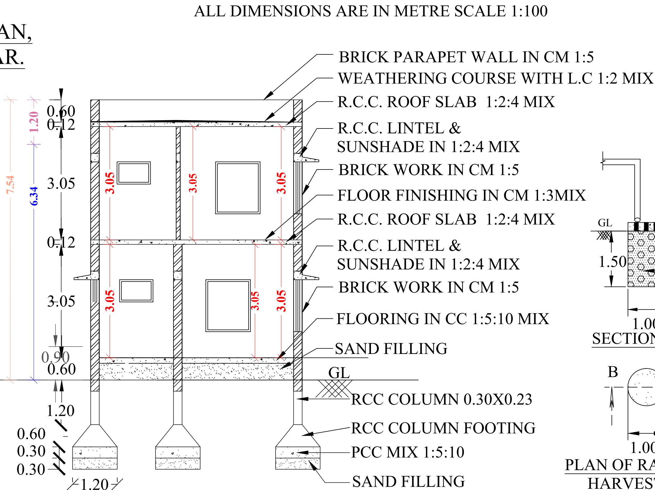
SECTION ON "BS"
