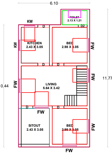
PLAN - GROUND FLOOR (PROPOSED)
