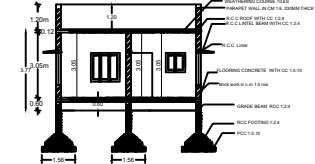
SECTIONON-AA
