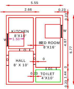
PRO FIRST FLOOR RESIDENTIAL PLAN
