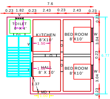
EXT GROUND FLOOR RESIDENTIAL PLAN
