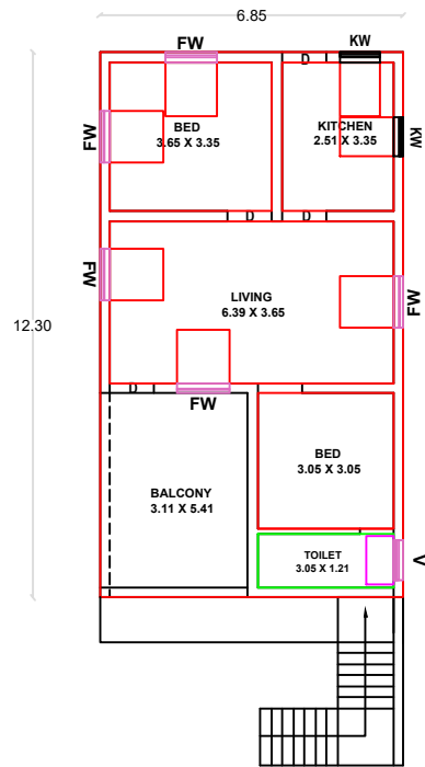
PLAN - FIRST FLOOR ( PROPOSED )
