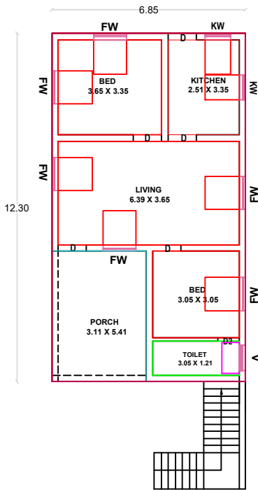
PLAN - GROUND FLOOR
