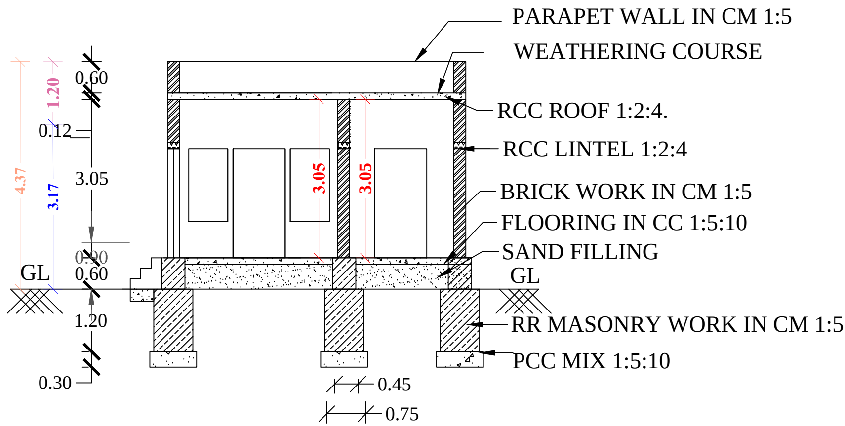
SECTION OF "AB"
