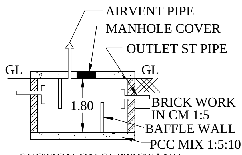
SECTION ON SEPTICTANK
