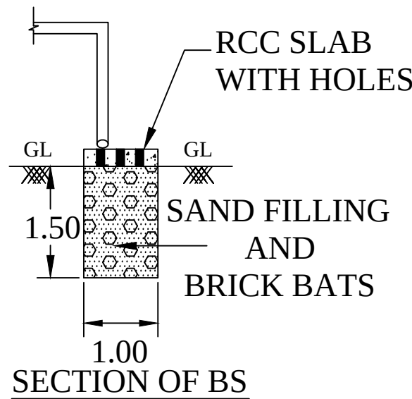
SECTION OF BS
