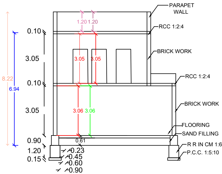
SECTION AB
