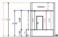
SECTION "A-A" (PROPOSED)
