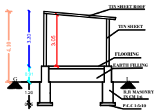
SECTION AB
