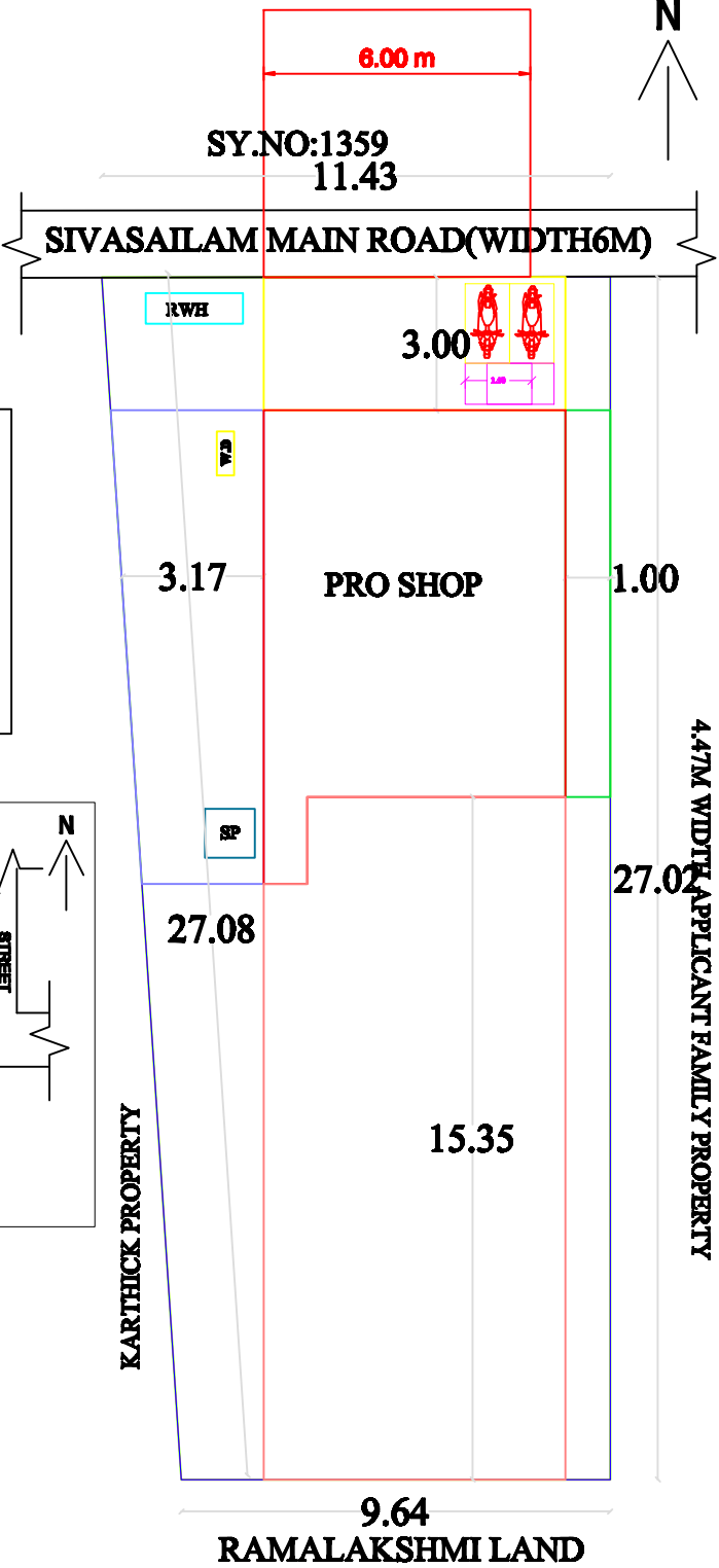
TOPO PLAN
