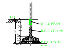
SECTION OF FOOTING
