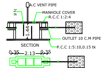
PLAN OF SEPTIC TANK &amp; TRENCH
