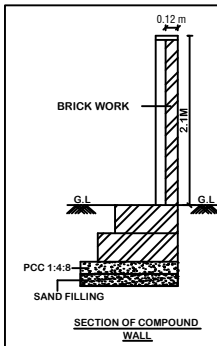
SECTION OF COMPOUND WALL
