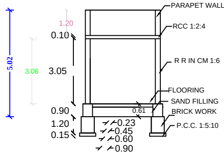
SECTION AB
