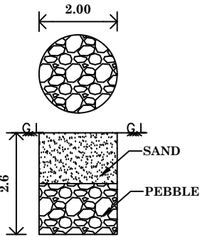
RAINWATER HARVESTING
