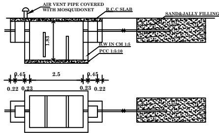
PLAN&SECTION OF SEPTIC TANK TRENCH
