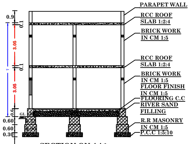
SECTION ON AA1
