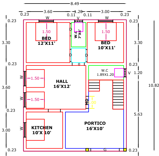
PRO GROUND FLOOR RESIDENTIAL PLAN
