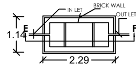
PLAN OF SEPTIC TANK
