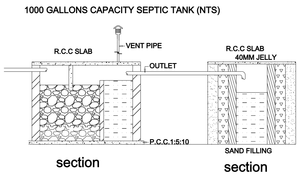
section
