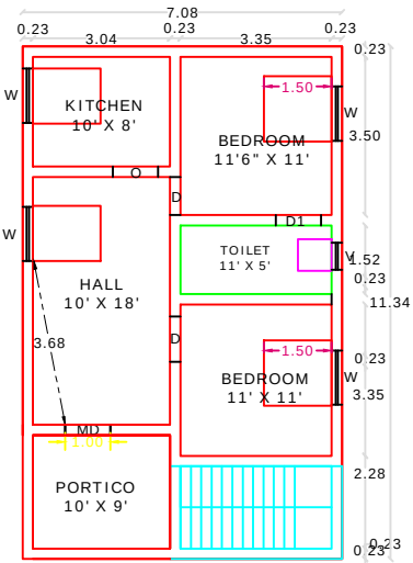
GROUND FLOOR RESIDENTIAL PLAN
