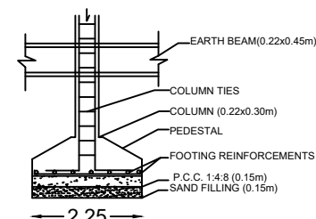
FOUNDATION DETAILS
