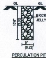
PERCOLATION PIT
