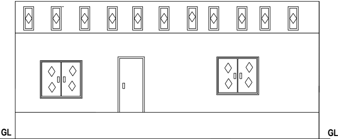
ELEVATION (PROPOSED)
