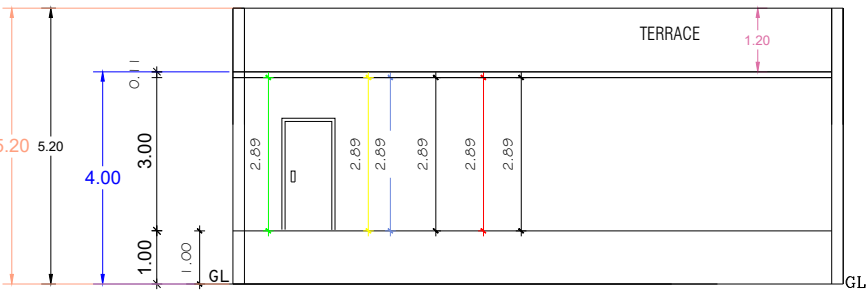
SECTION "A-A" (PROPOSED)
