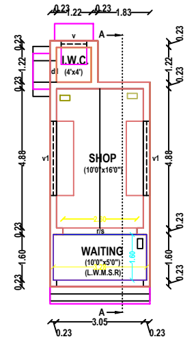
PLAN - GROUND FLOOR SHOP
