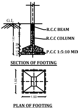
COLUMN DETAILS
