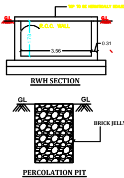
RWH DETAILS
