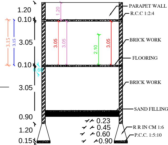
SECTION AB
