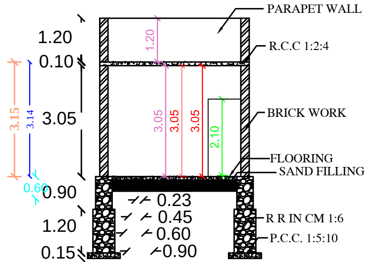
SECTION-AB
