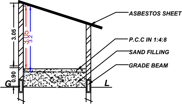
SECTION "AB"
