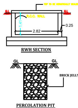
PERCOLATION PIT
