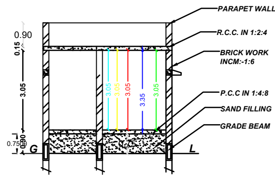
SECTION "AB"
